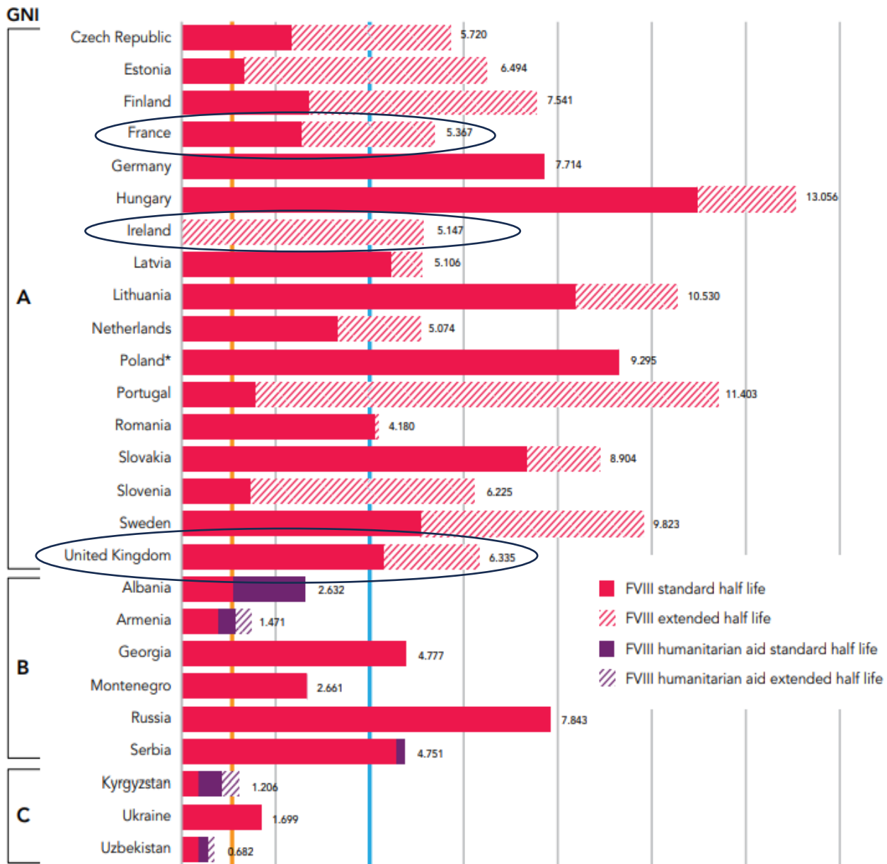
FIGURE G4a. Mean per capita factor VIII use in 2021 – regional and GNI comparisons of IU/total population: Europe
